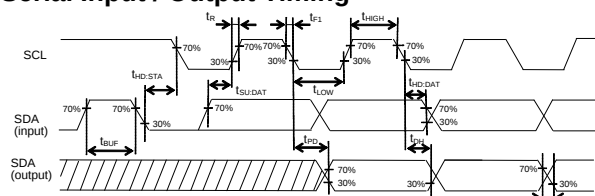
Figure 2-(a). Serial Input / Output Timing
