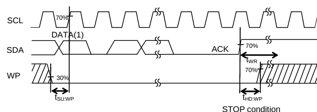
Figure 2-(d). WP Timing at Write Execution
