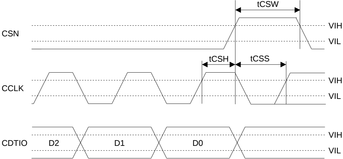
Figure 15. WRITE Data Input Timing (3-wire Serial: AK4951EG)
