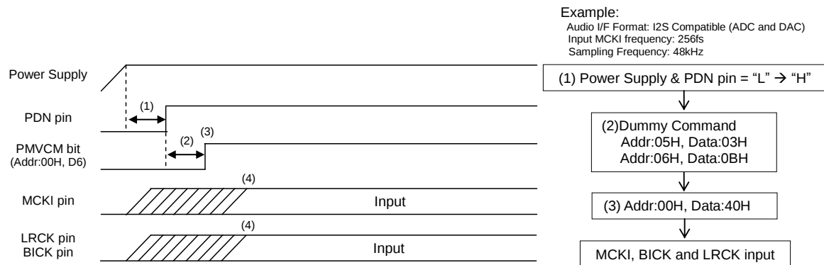
Figure 70. Clock Set Up Sequence (3)
