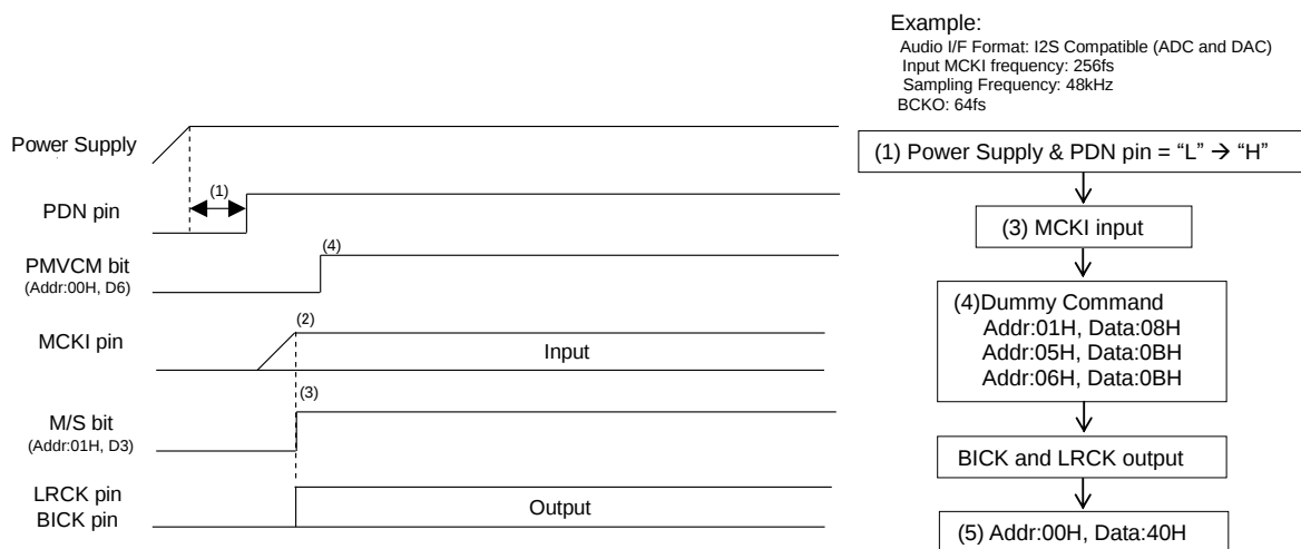
Figure 71. Clock Set Up Sequence (4)
