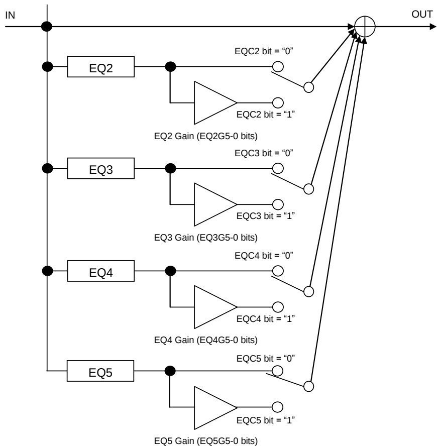
Figure 42. 4-Band EQ Structure
