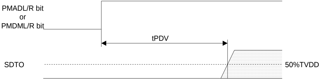
Figure 18. Power Down & Reset Timing 2
