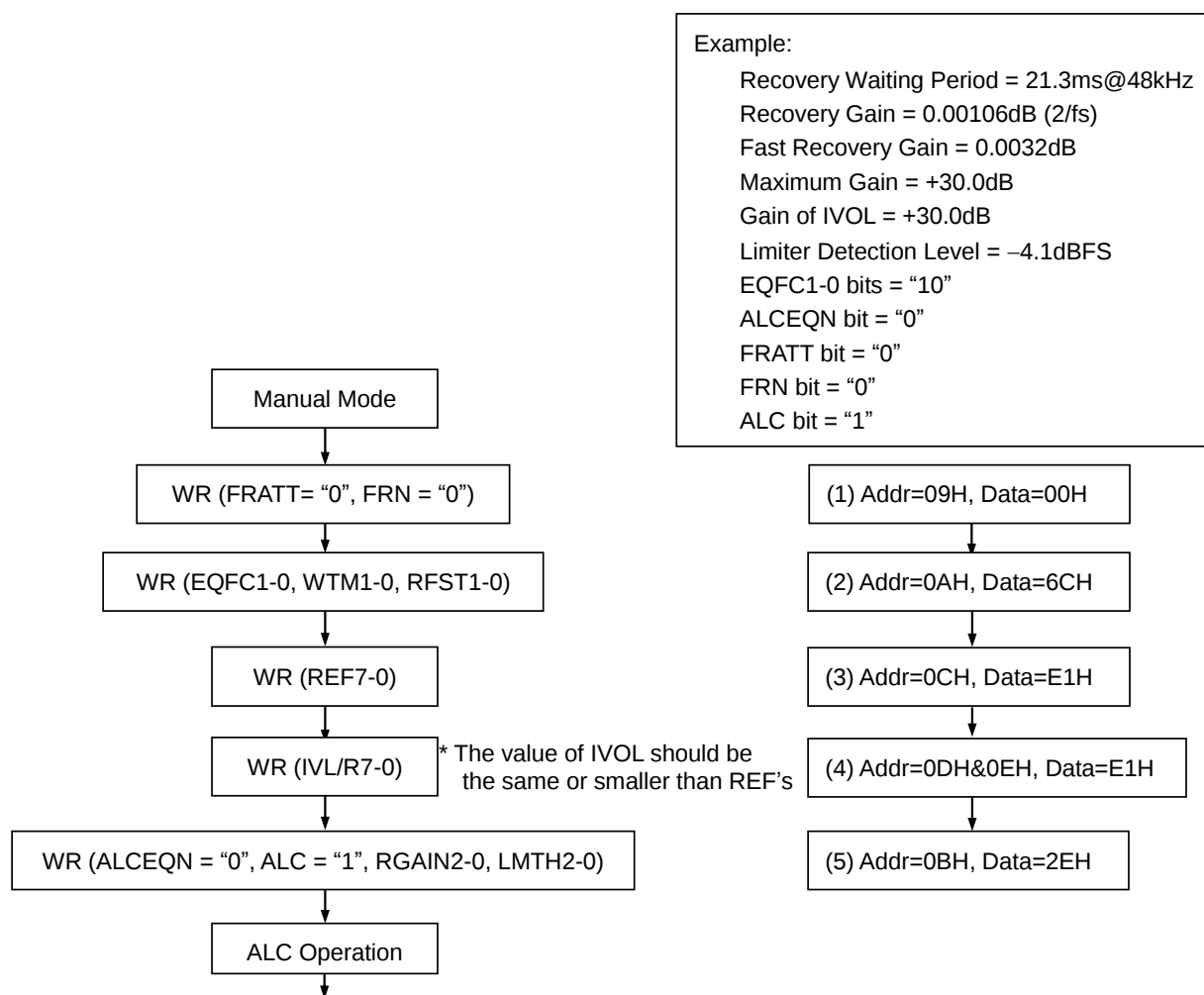
Figure 45. Registers Set-up Sequence at ALC Operation (Recording path)
