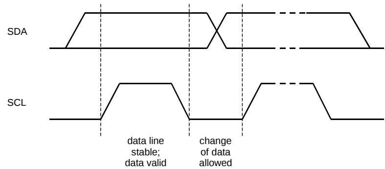
Figure 63. Bit Transfer (I 2 C Bus)
