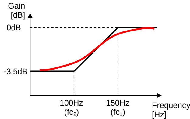
Note 42. Black: Diagrammatic Line, Red: Actual Curve Figure 44. ALCEQ Frequency Response ( fs = 48\text{kHz} )
