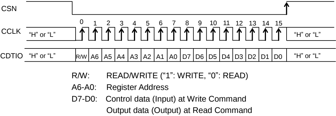
Figure 64. Serial Control Interface Timing 1
