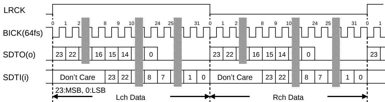
Figure 27. Mode 0 Timing
