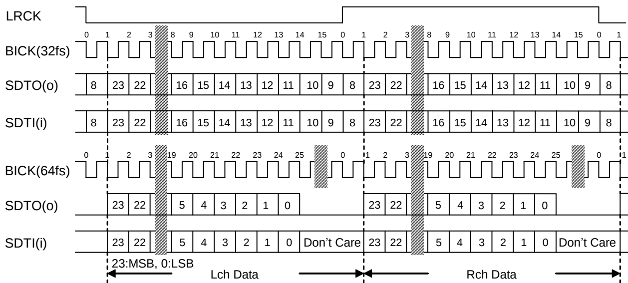
Figure 30. Mode 3 Timing
