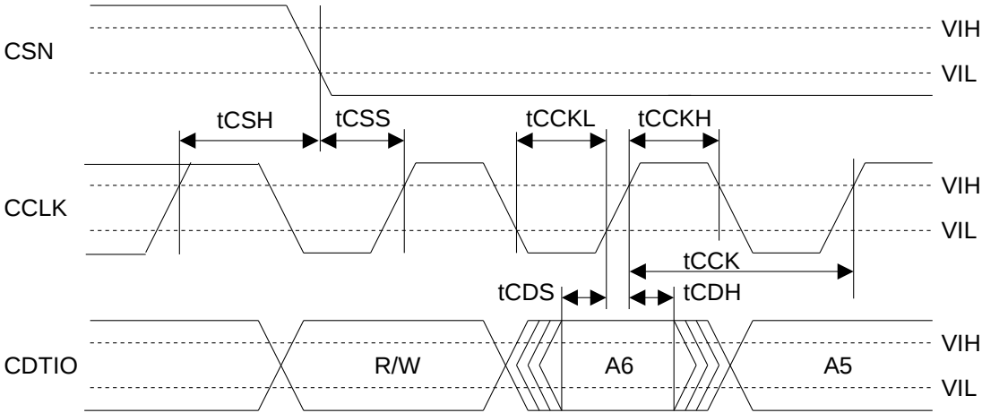
Figure 14. WRITE Command Input Timing (3-wire Serial: AK4951EG)
