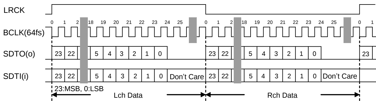
Figure 29. Mode 2 Timing
