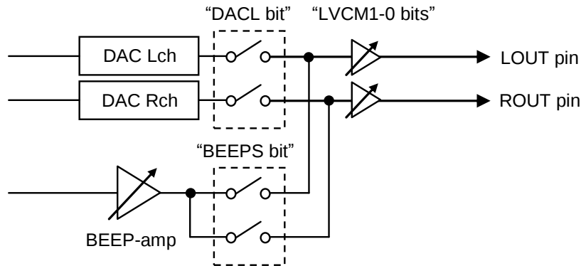
Figure 50. Stereo Line Output
