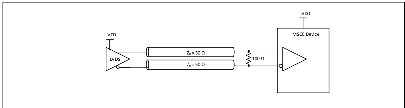
Figure 8. Input driven by LVDS output
