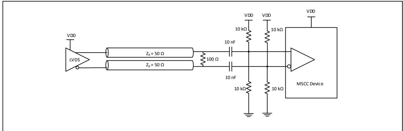
Figure 9. Input driven by AC coupled LVDS
