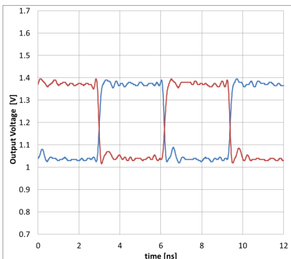
Figure 17. 156.25MHz LVDS
