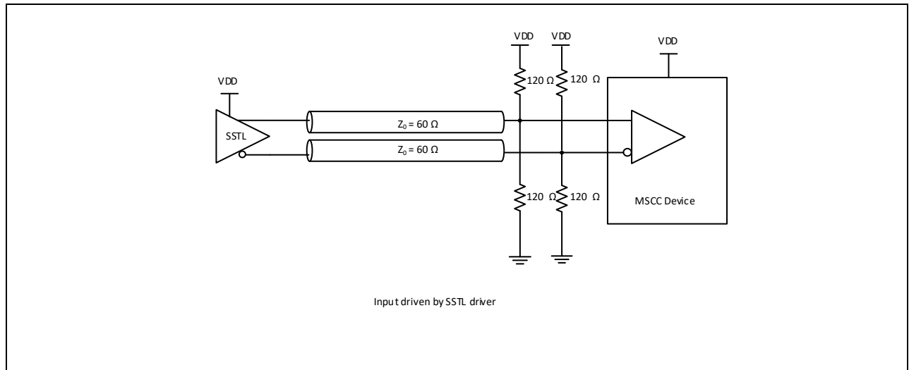
Figure 10. Input driven by an SSTL output
