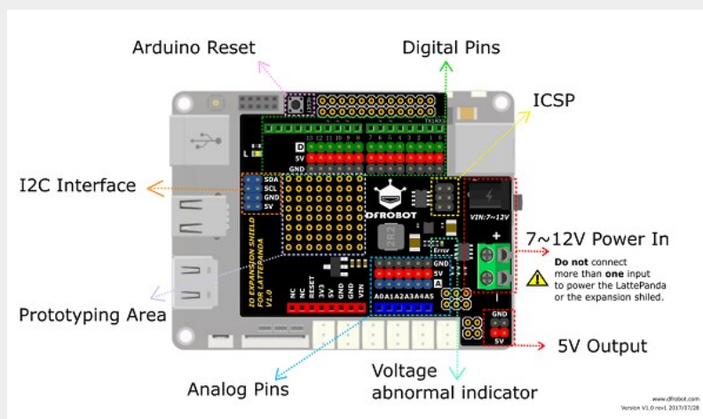
Gravity IO Expansion Shield for LattePanda Pinout
