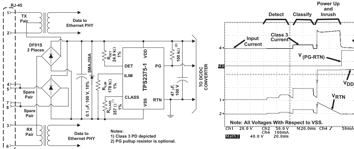
Figure 1. Typical Application Circuit and Start-Up Waveforms
