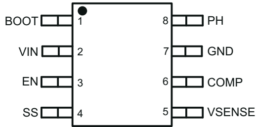
Figure 5-1. 8-Pin SOIC D Package (Top View)
