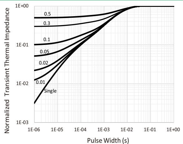
Figure 8: Transient Thermal Impedance (Per Component)
