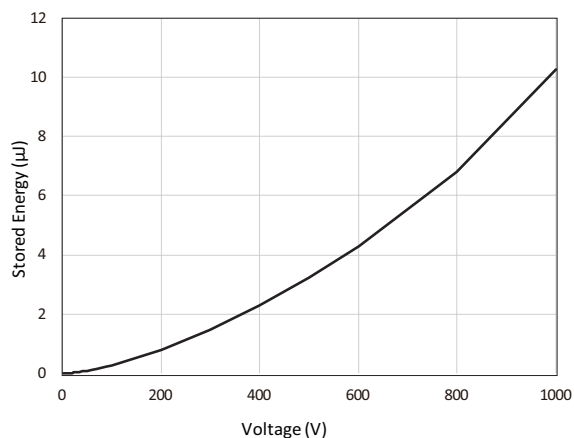
Figure 7: Stored Energy vs. Reverse Voltage (Per Leg)
