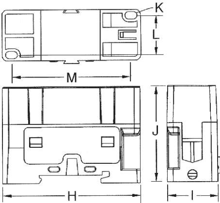
100 amp holder
