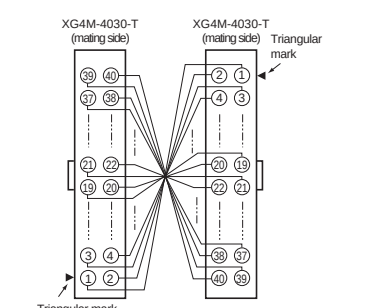
Wiring Diagram
