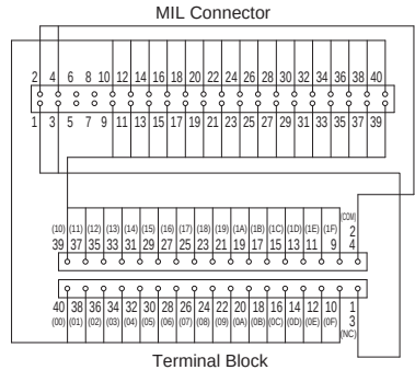
XW2R-P34GD-M1
