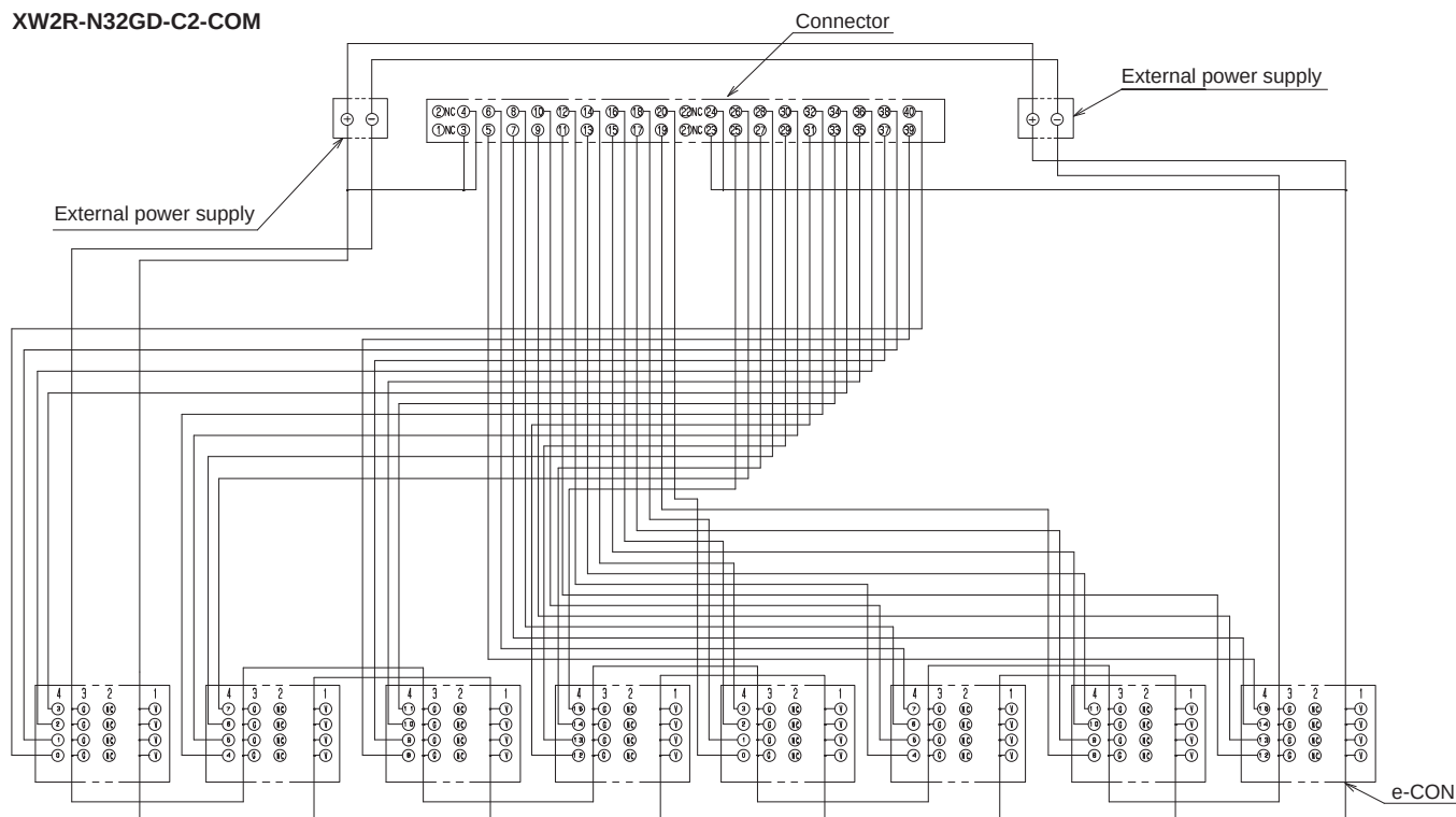
XW2R-N32GD-C2-COM
