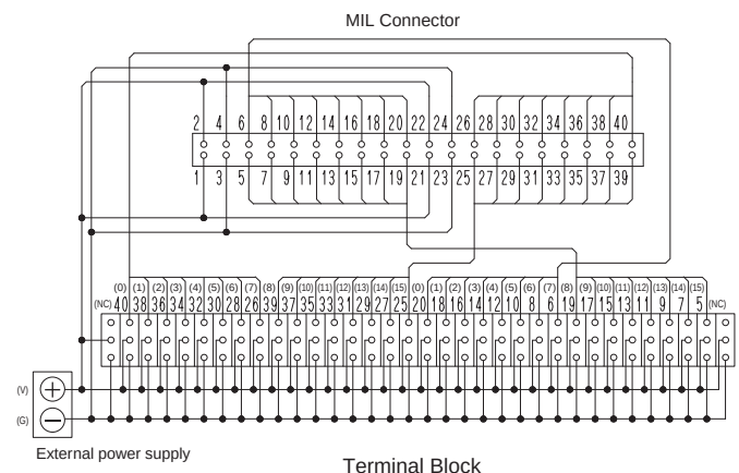
XW2R-P32GD-C4-COM
