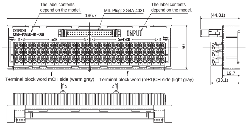
XW2R-P32GD-M1-COM
