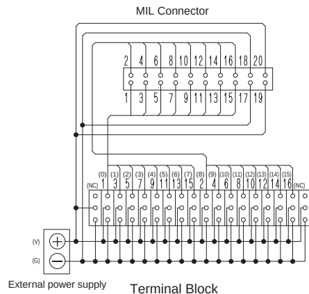
XW2R-P16GD-C3-COM
