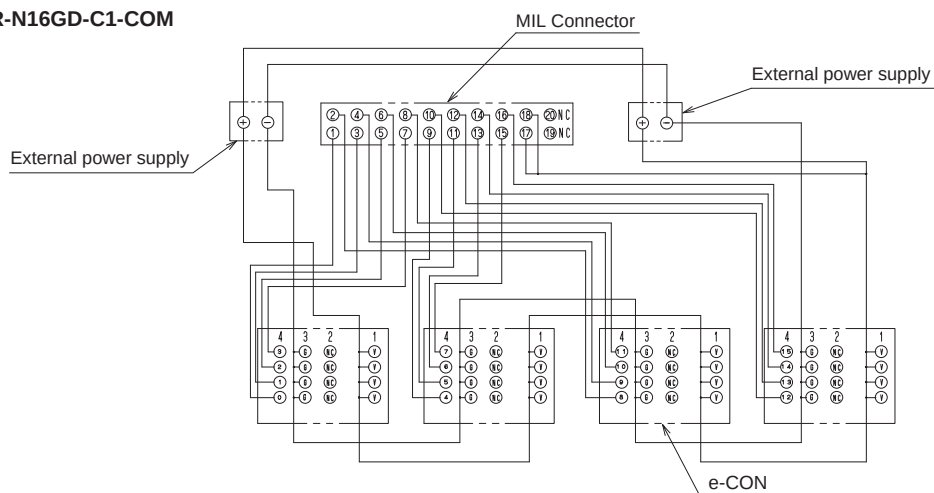
XW2R-N32GD-C1-COM
