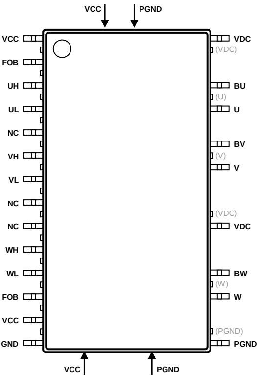
Figure 39. Dummy Pins
