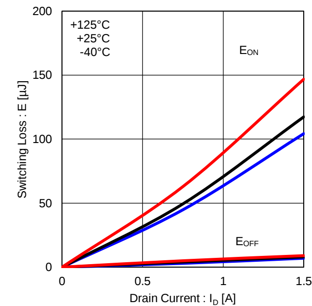
Figure 36. Low Side Switching Loss (VDC=300V)
