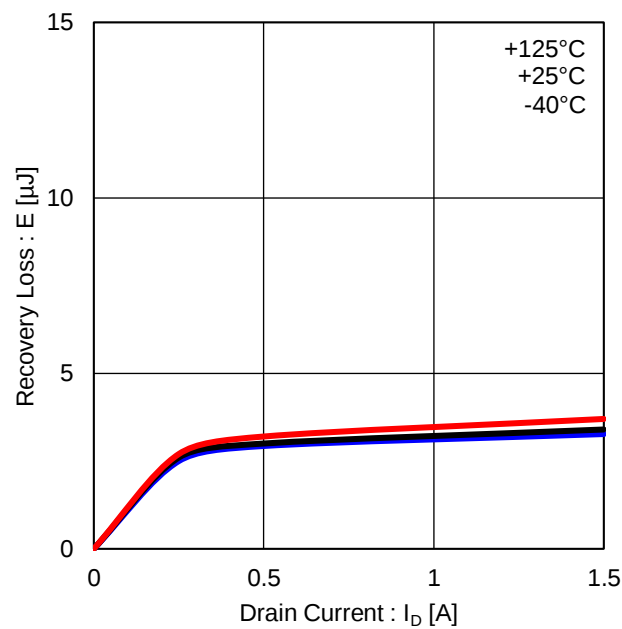
Figure 37. Low Side Recovery Loss (VDC=300V)
