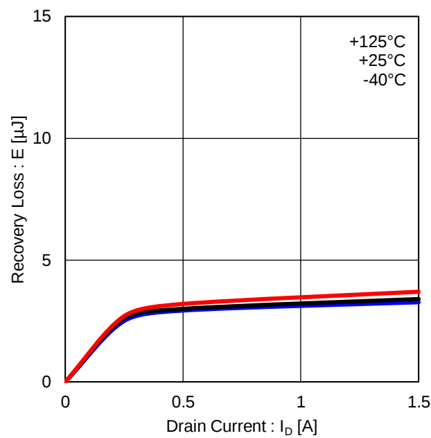
Figure 35. High Side Recovery Loss (VDC=300V)
