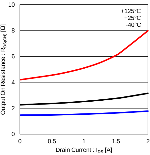
Figure 30. Output MOSFET ON Resistance
