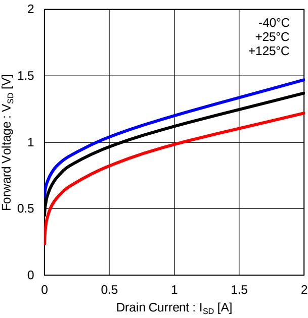
Figure 31. Output MOSFET Body Diode
