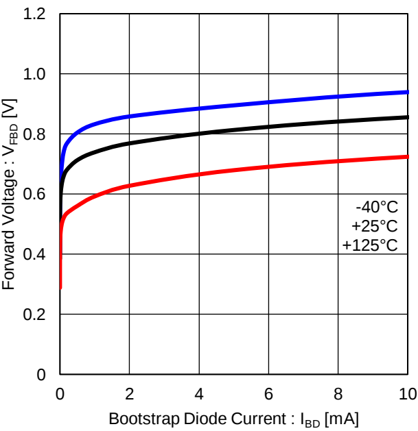
Figure 32. Bootstrap Diode Forward Voltage
