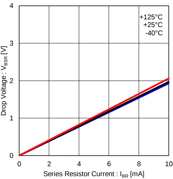
Figure 33. Bootstrap Series Resistor
