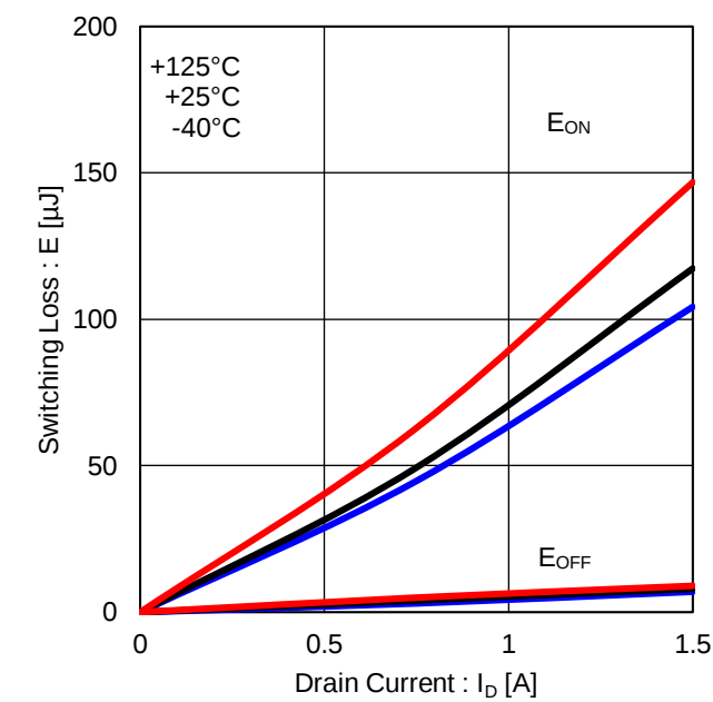
Figure 34. High Side Switching Loss (VDC=300V)
