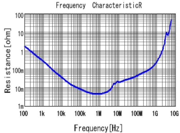
■ GRT31CR61E335KE01 R DC0V, 25degC
