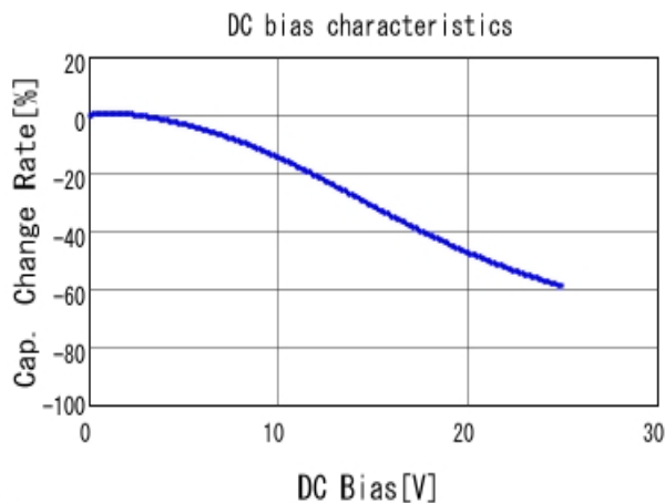
■ GRT31CR61E335KE01 C-DC bias capchange, 25.0degC, AC1.
