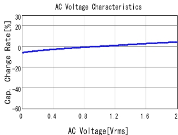
■ GRT31CR61E335KE01 C-AC Voltage capchange, DC0V, 25.0d
