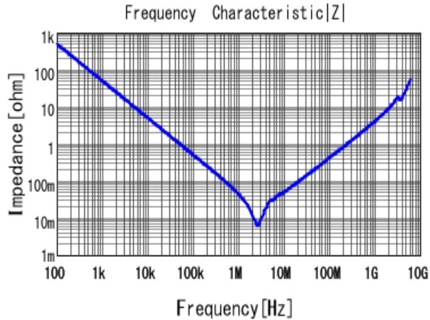
■ GRT31CR61E335KE01 |Z| DC0V, 25degC
