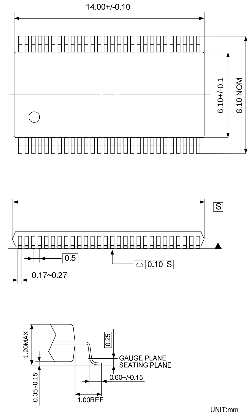
Figure 16. Package Diagram
