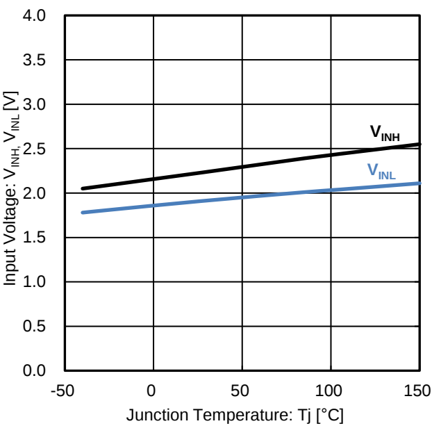
Figure 11. Input Voltage vs Junction Temperature
