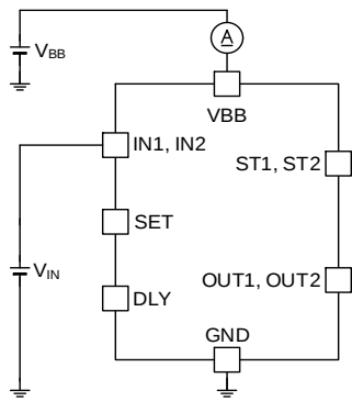
Figure 25. Operating Current
