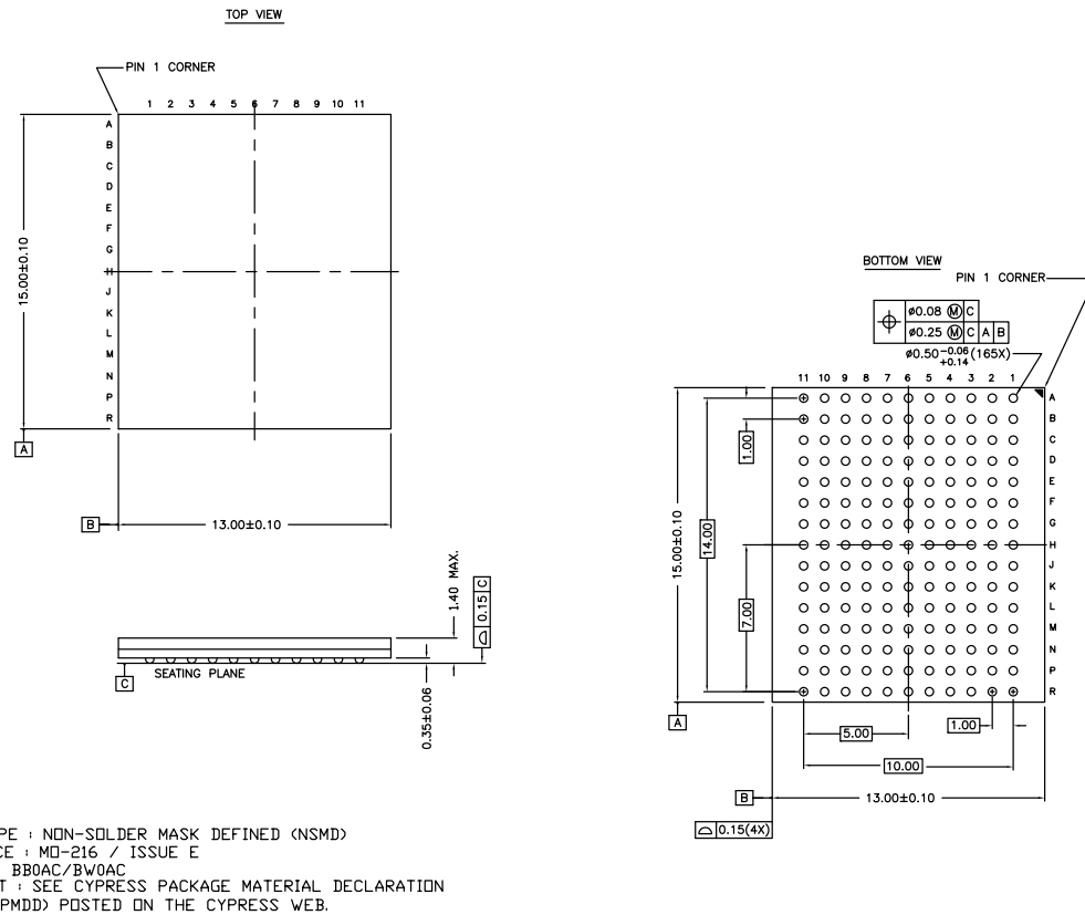
Figure 6. 165-ball FBGA (13 × 15 × 1.4 mm) BB165D/BW165D (0.5 Ball Diameter) Package Outline, 51-85180
