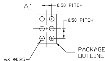
RECOMMENDED MOUNTING FOOTPRINT*
