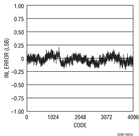
Typical INL, 2V Range
