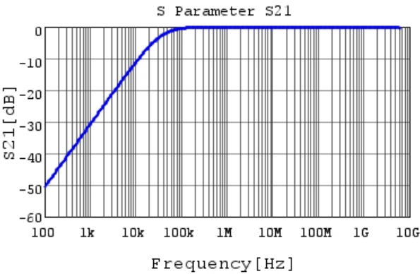
GCJ188R71H473KA12 S21 DC0V,25degC
