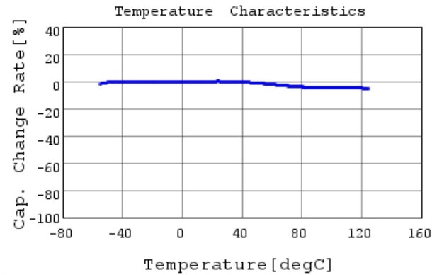
GCJ188R71H473KA12 C-Temp. capchange, DC0.0V,
