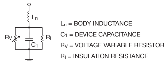
Figure 4. Antenna Varistor
