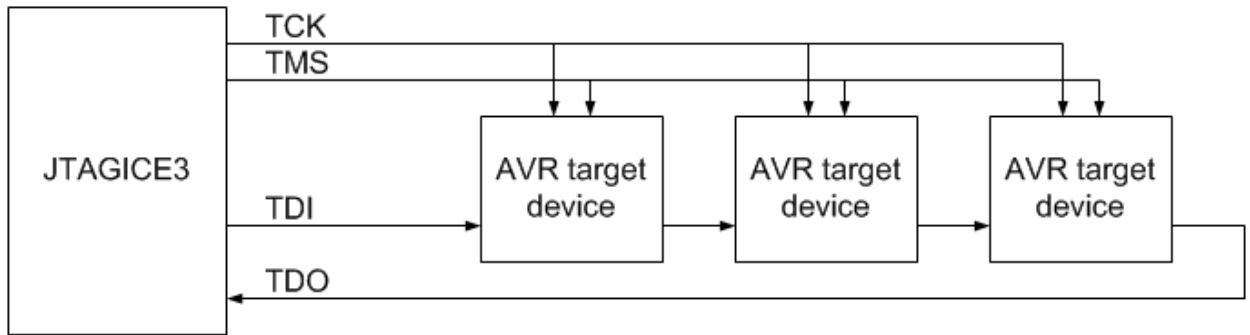
Figure 4-3. JTAG Daisy-chain
