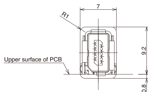
Reference housing panel cut-out dimension (FREE)
