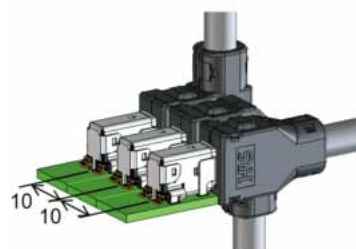
Parallel mounting on a narrow pitch (P=10mm)
