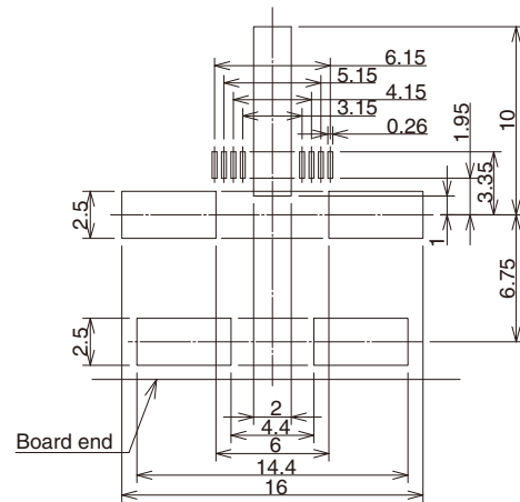
Recommended metal mask pattern (t=0.1mm)
