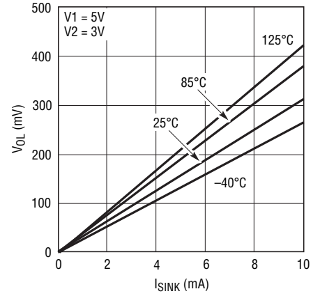
Voltage Output Low vs Output Sink Current ( RST , COMP_n )
