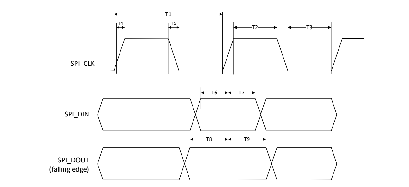
Figure 44: gSPI Timing
