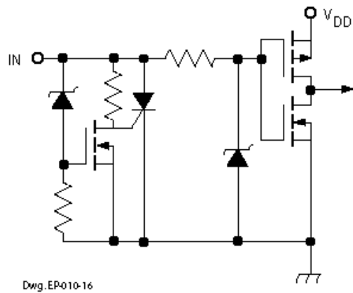
LOGIC INPUTS
