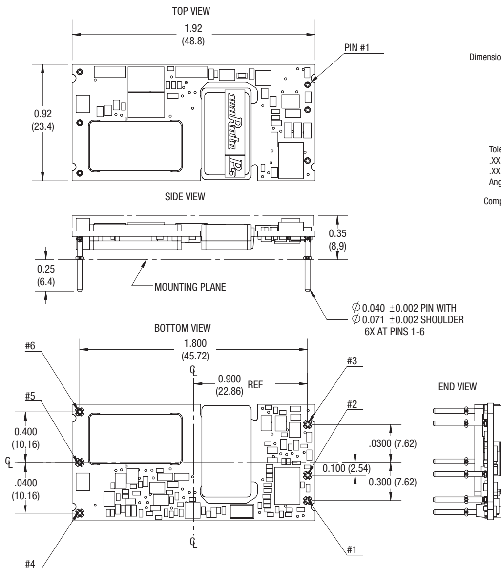
UEI30 Open Frame 30W Package C80
