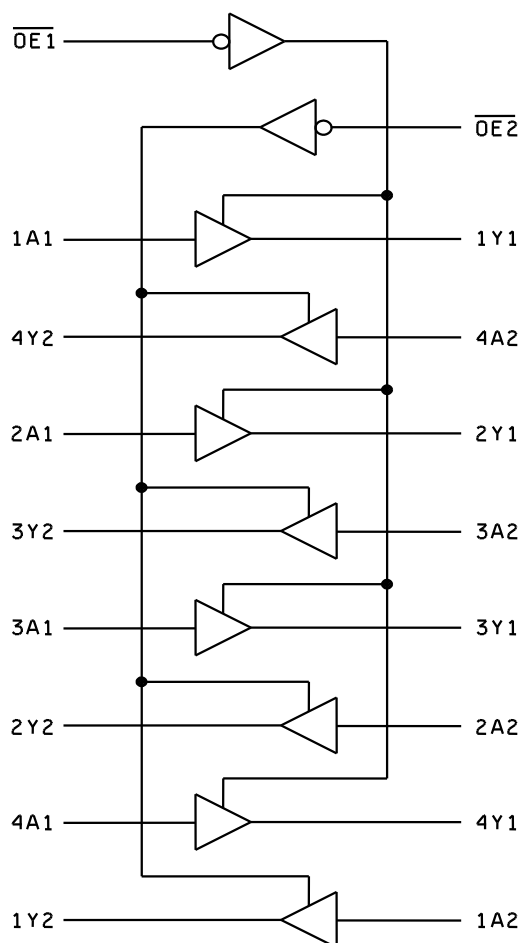
FIGURE 4. Logic diagram.
