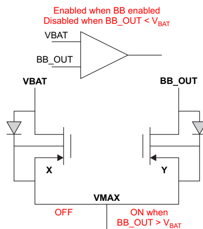
Figure 70. VMAXx_DIS: 1, VMAXx_EN: 0, VMAX_LATCH: 1
