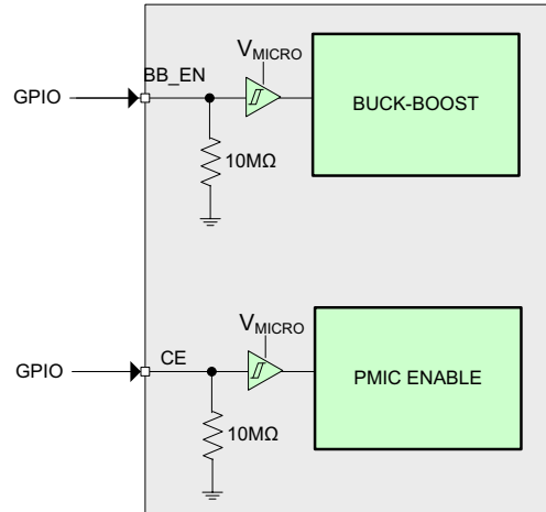
Figure 65. Power Up and Enabling the IC
