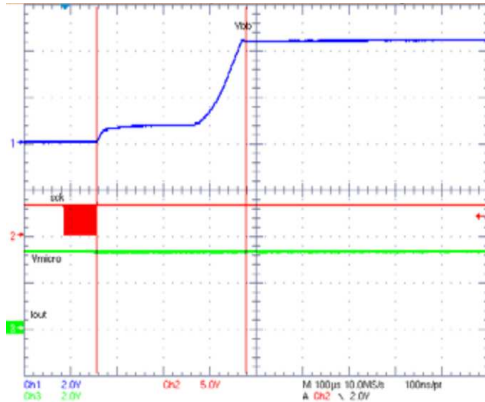
Ch1: BB output Ch2: I²C SCLK turns on buck-boost Ch3: VMICRO Start-up time is 330 \mu\text{s} Buck-Boost L and C are per application circuit
