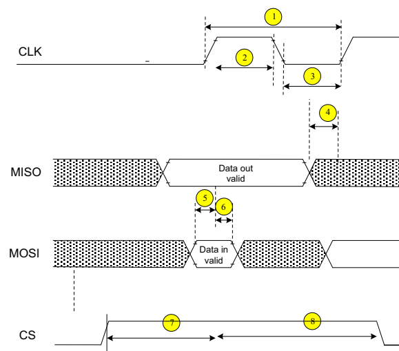
Figure 1. Timing Diagram
