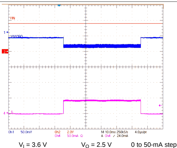
Figure 39. BUCK MINI Transient Response
