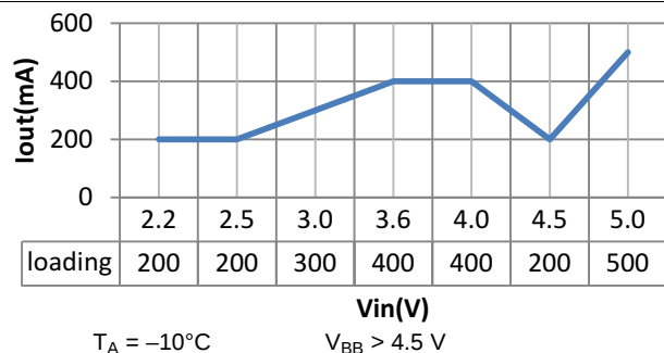
Figure 11. Buck-Boost Loading
