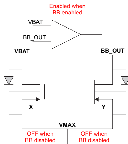
Figure 68. VMAXx_DIS: 1, VMAXx_EN: 0, VMAX_LATCH: 0
