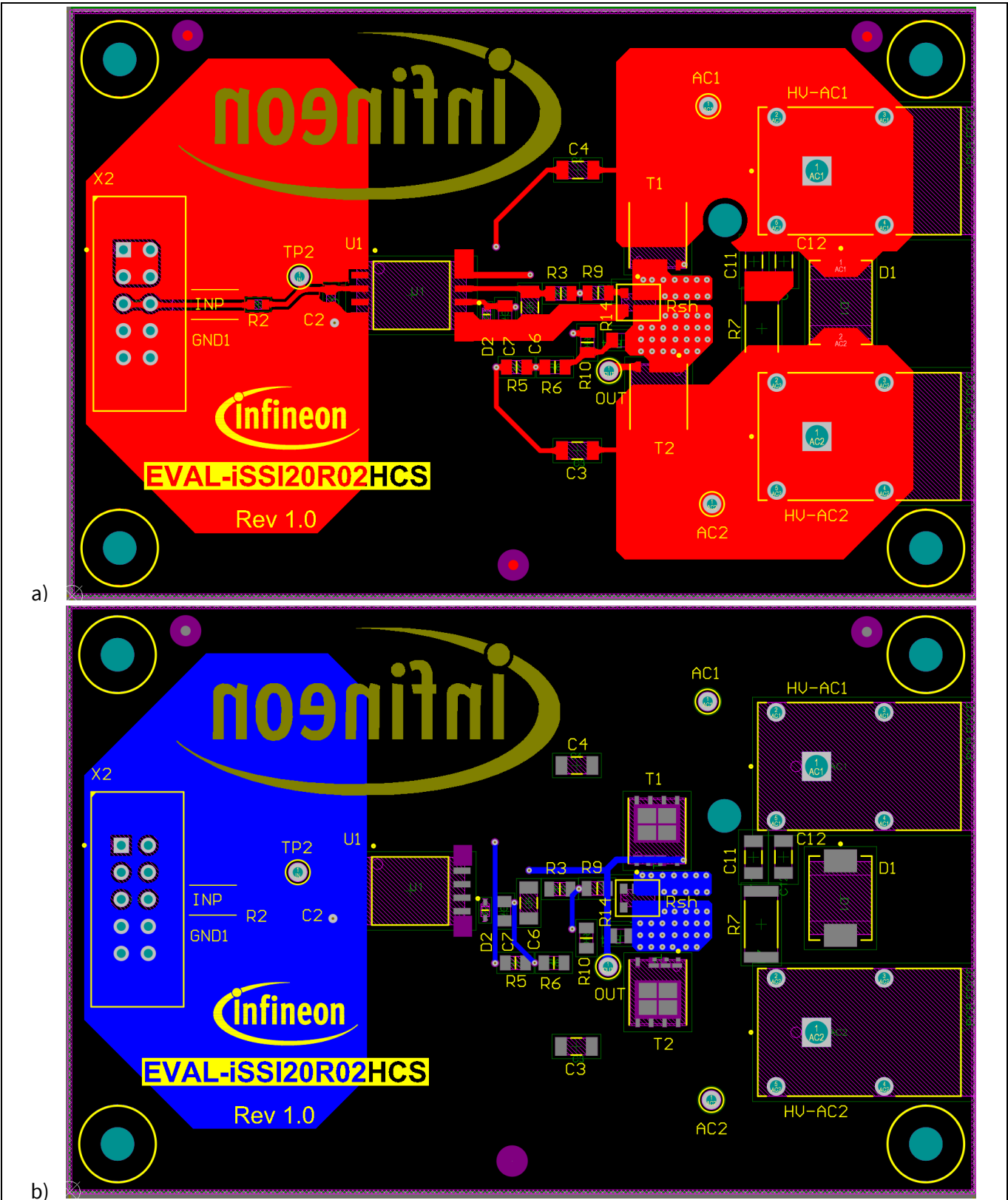
Figure 4 Top (a) and bottom (b) layers of EVAL-iSSI20R02HCS
