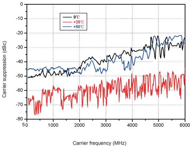
Measured carrier suppression
