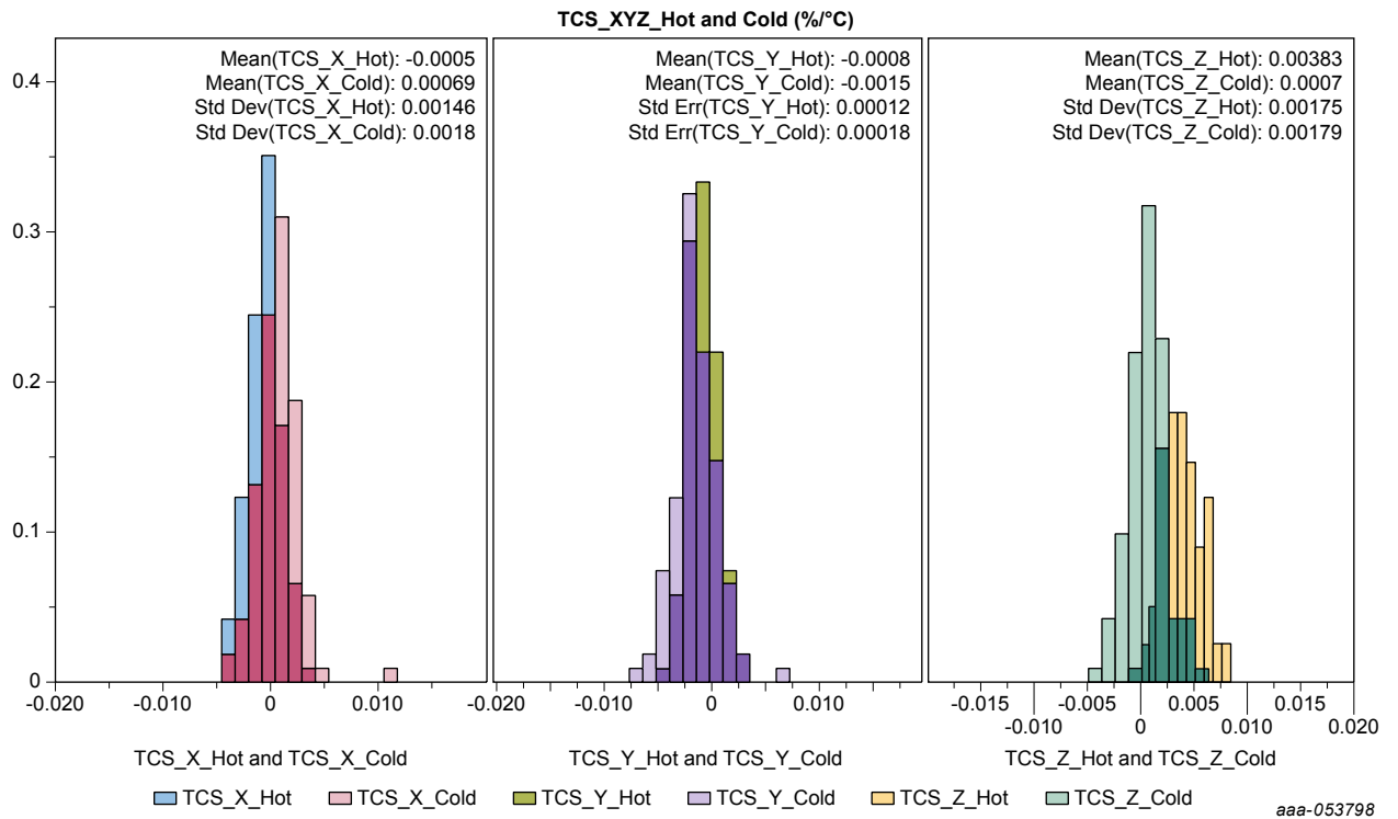
Figure 6. XYZ_TCS histograms
