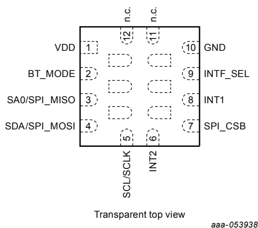
Figure 2. Pin configuration diagram
