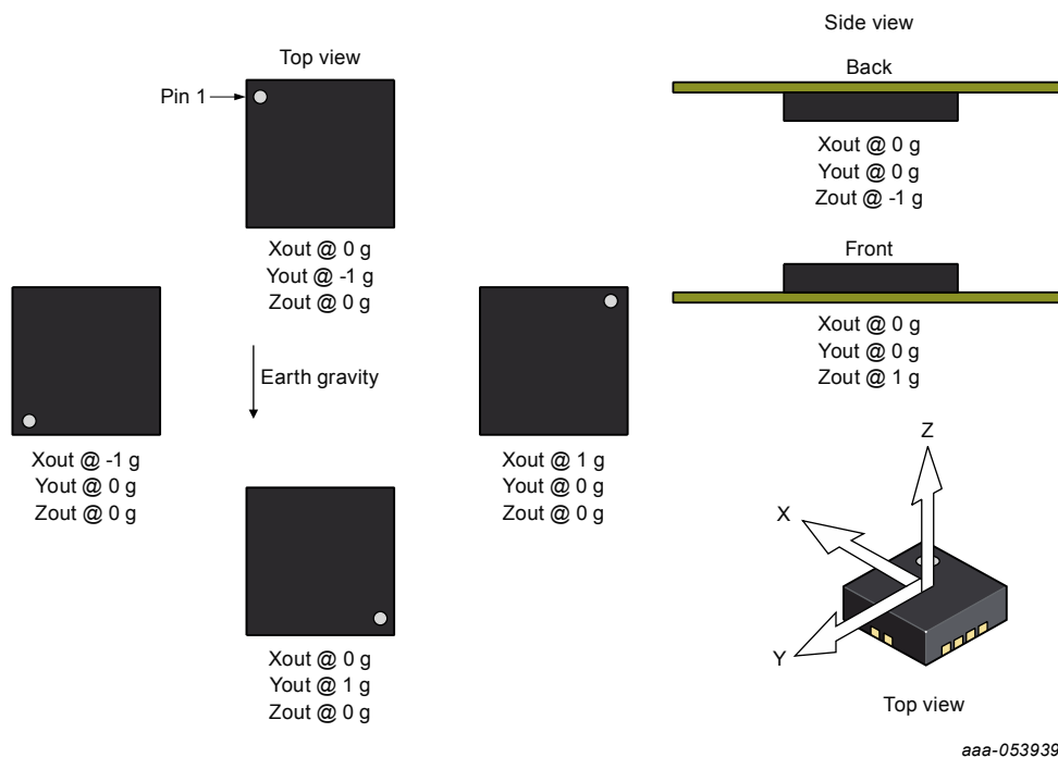
Figure 3. Sensitive axes orientation and output response to \pm 1 g (gravity) stimulus
