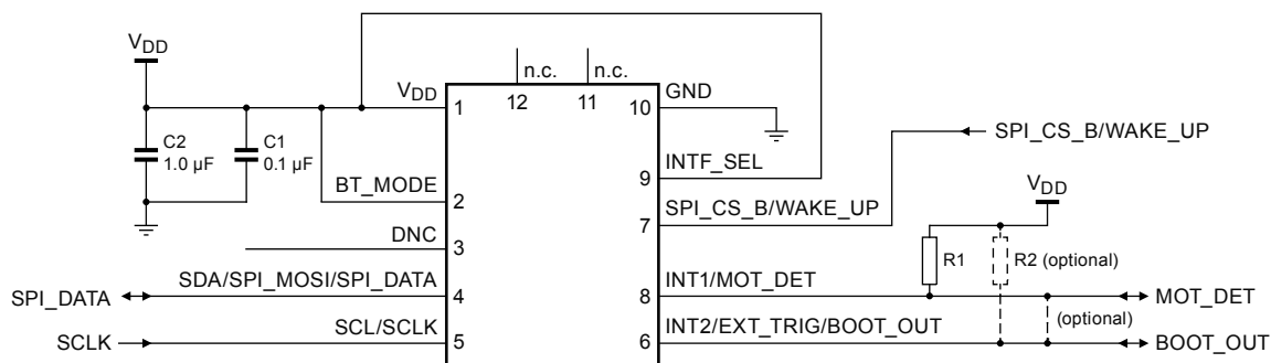
Figure 27. Typical Application Circuit #6 - Motion detection mode (with SPI 3-wire interface, software enabled)
