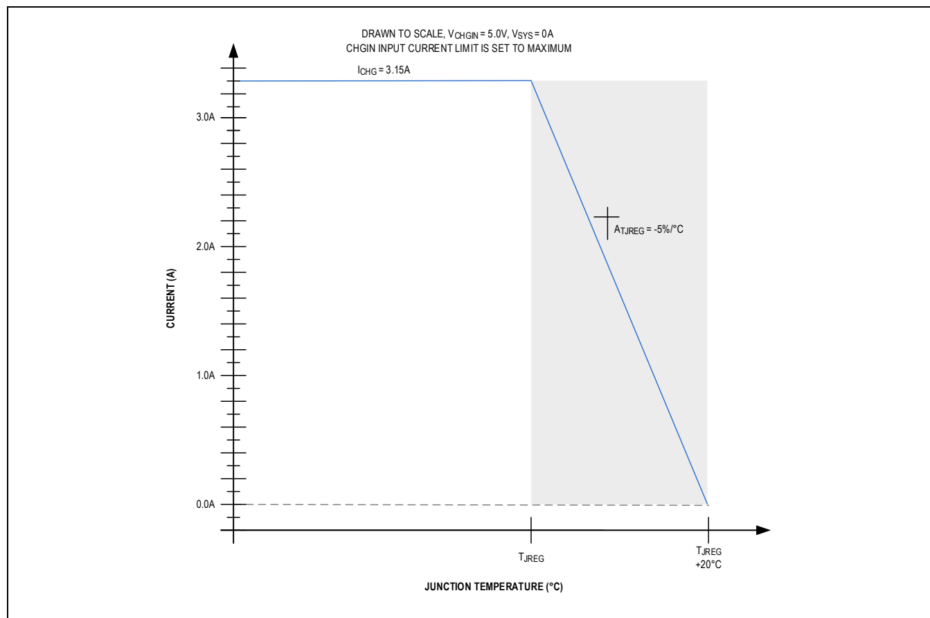
Figure 8. Charge Currents vs. Junction Temperature
