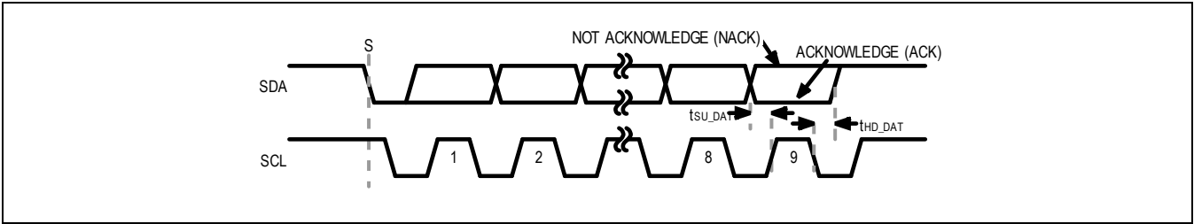
Figure 23. Acknowledge Bit
