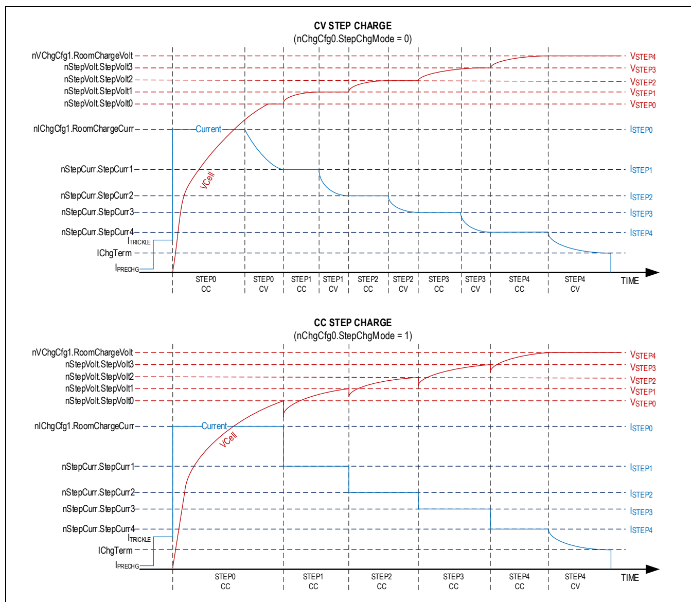
Figure 3. Step-Charging State Machine
