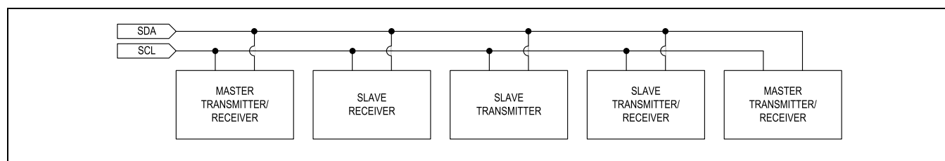
Figure 21. I 2 C System Configuration
