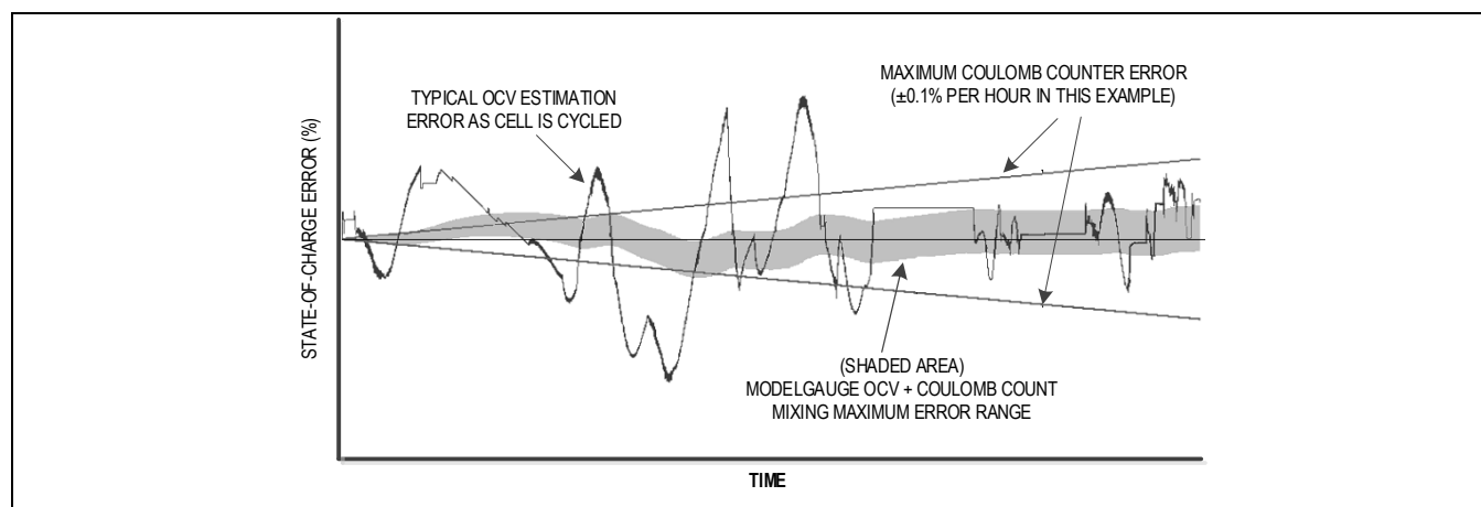
Figure 13. ModelGauge m5 Typical Accuracy Example
