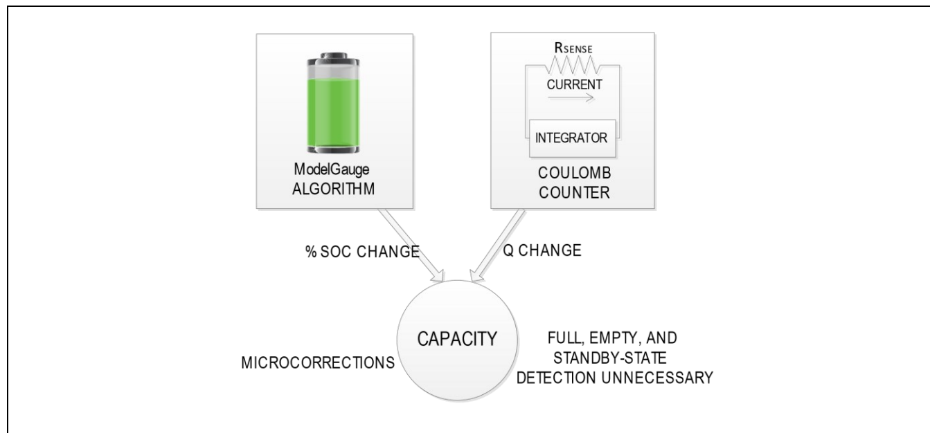
Figure 9. ModelGauge m5 Algorithm
