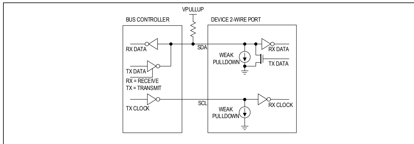
Figure 20. I 2 C Simplified Block Diagram
