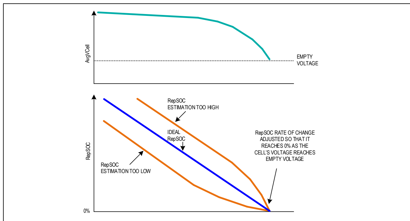
Figure 17. Converge-To-Empty Performance
