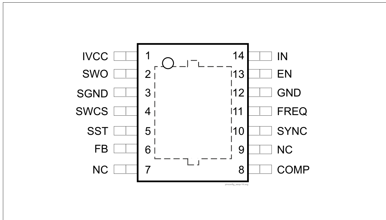
Figure 2 Pin Configuration
