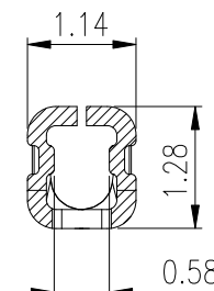
SEC C-C SCALE 2:1
