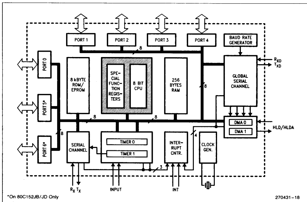
Figure 2. Block Diagram
