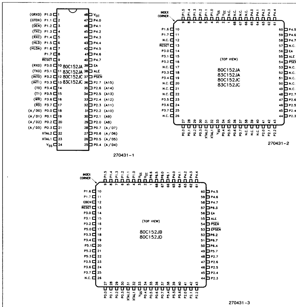
Figure 1. Connection Diagrams
