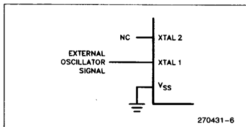
Figure 4. External Clock Drive
