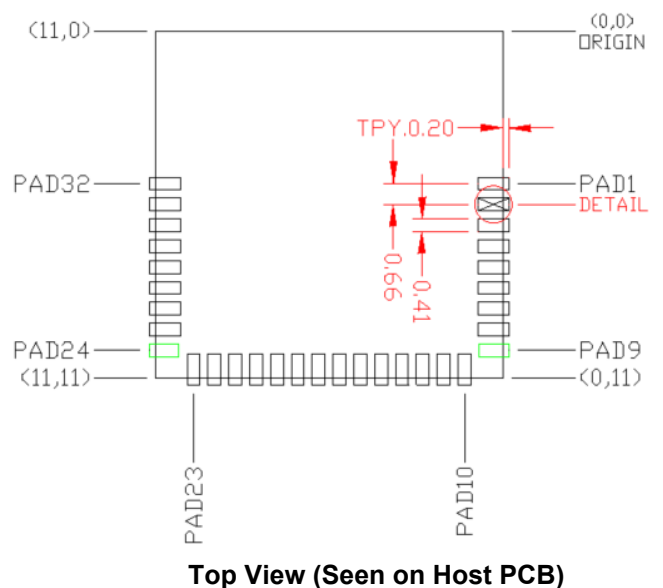
Figure 6. Solder Pad Reference Location
