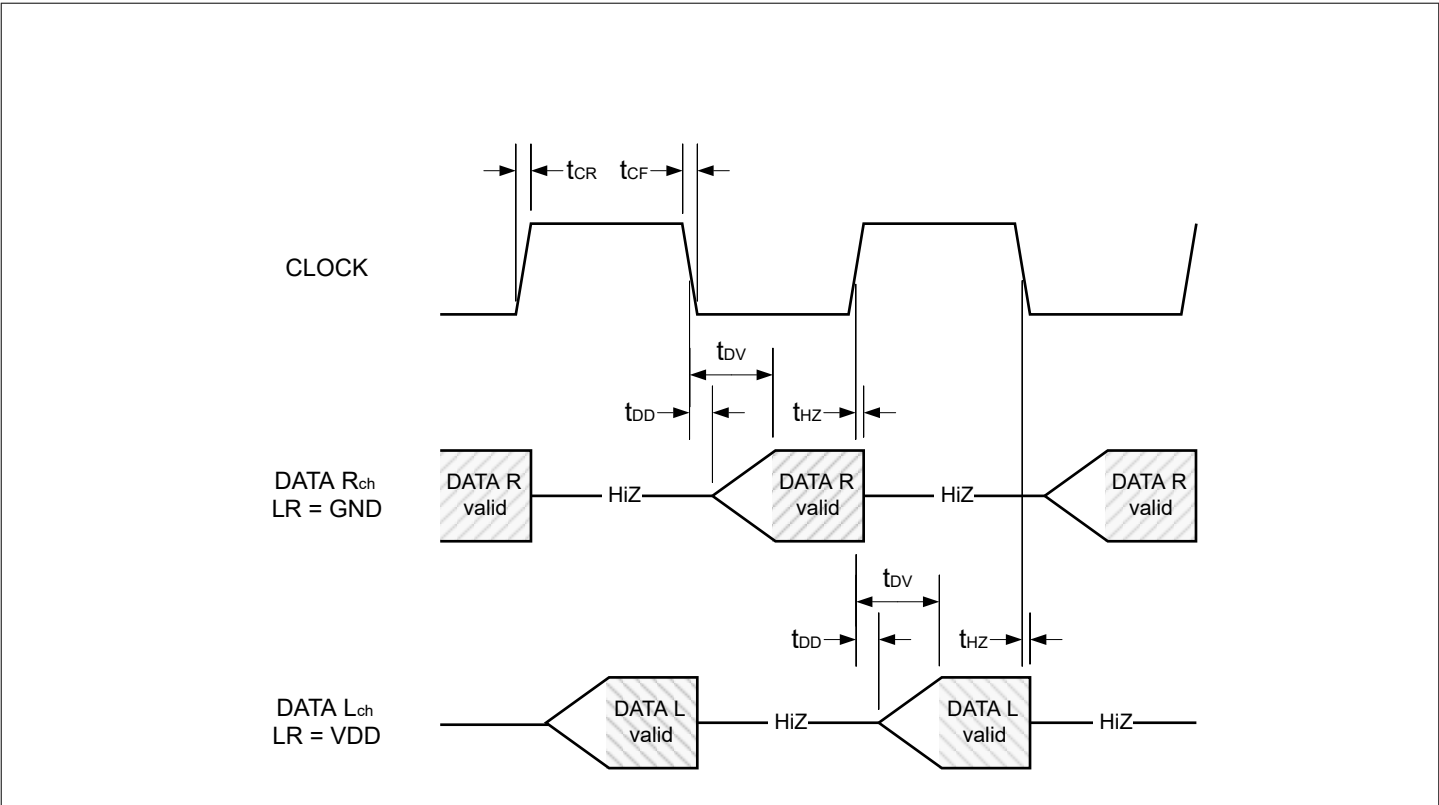
Figure 11 Timing diagram
