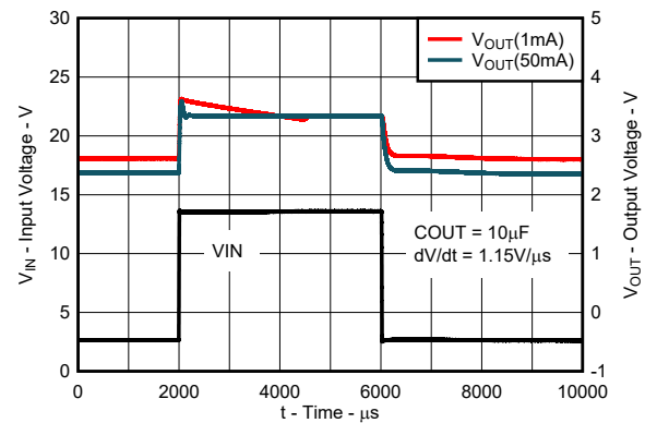
Figure 5-32. Line Transient Response (New Chip)
