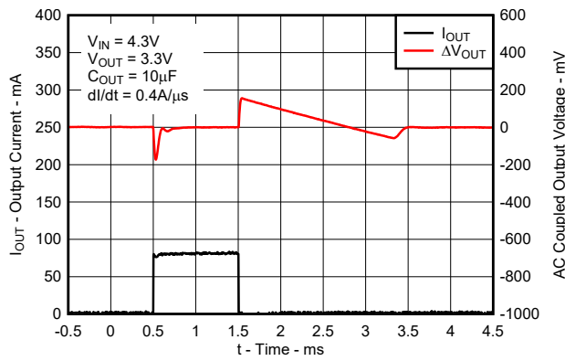
Figure 5-31. Load Transient Response (New Chip)
