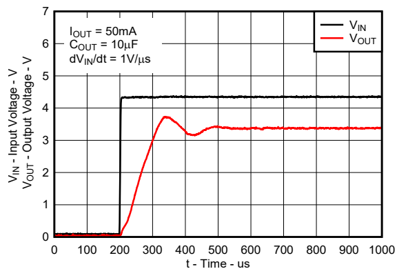
Figure 5-26. Fast Power-Up (Legacy Chip)
