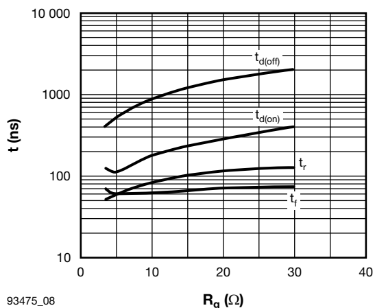
Fig. 8 - Typical Switching Times vs. Gate Resistance V_{CC} = 600 V, I_C = 300 A, V_{GE} = \pm 15 V, T_J = 125 ^{\circ}\text{C}
