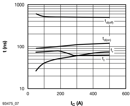
Fig. 7 - Typical Switching Times vs. I_C V_{CC} = 600 V, R_g = 4.7 \Omega , V_{GE} = \pm 15 V, T_J = 125 ^{\circ}\text{C}
