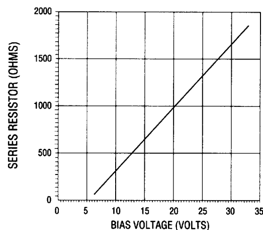
FIGURE 3 - SERIES LIMIT BIAS RESISTOR VS BIAS VOLTAGE
