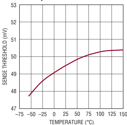
SENSE Current Limit Threshold vs Temperature
