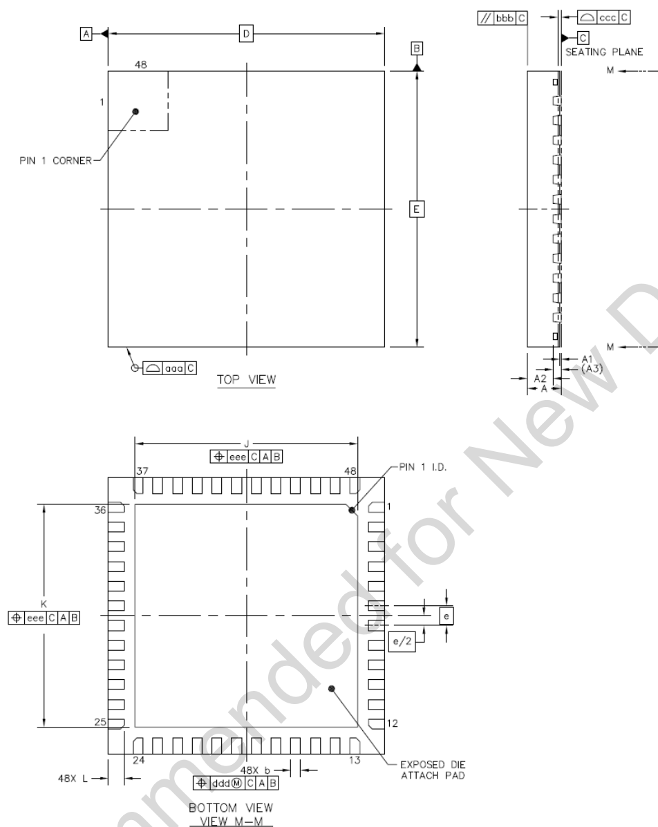
Figure 5.2. QFN48
