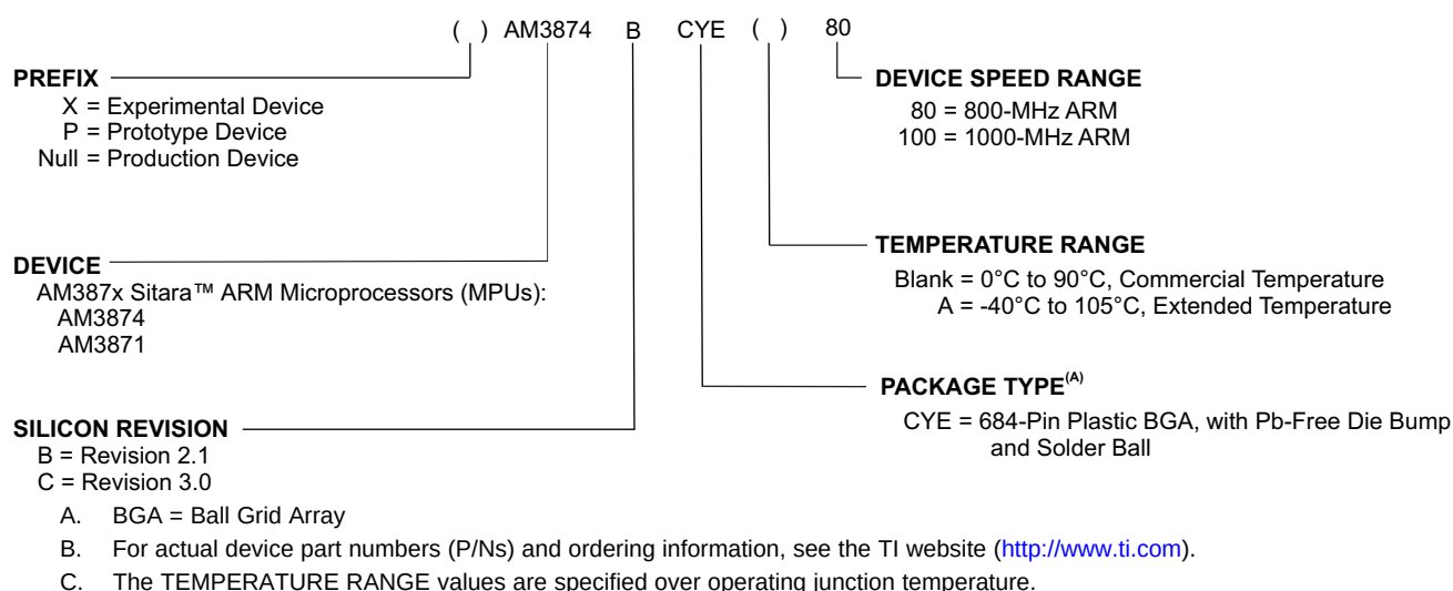
Figure 10-1. Device Nomenclature (B)(C)
