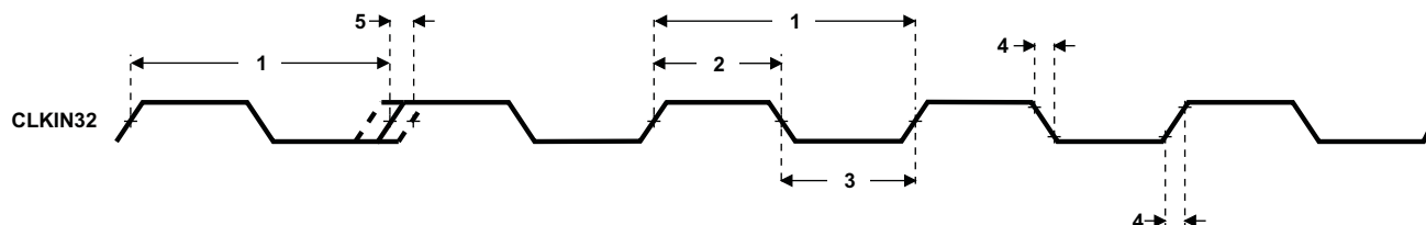
Figure 8-15. CLKIN32 Timing
