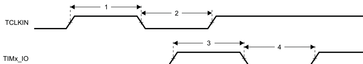
Figure 9-94. Timer Timing
