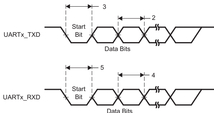
Figure 9-95. UART Timing
