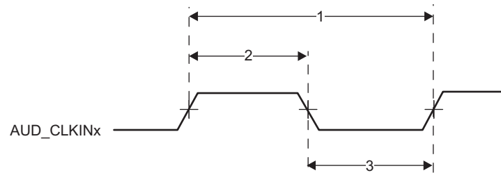
Figure 8-14. AUD_CLKINx Timing
