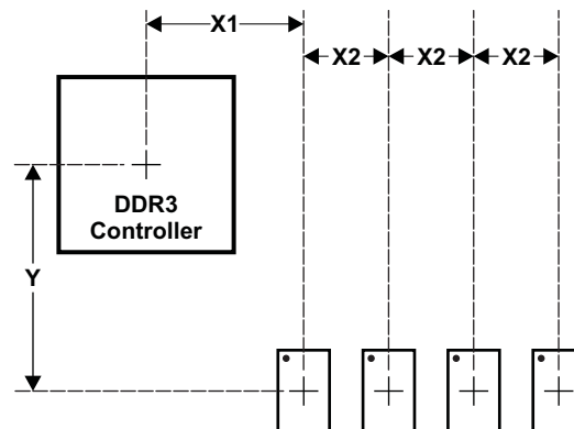
Figure 9-56. Placement Specifications
