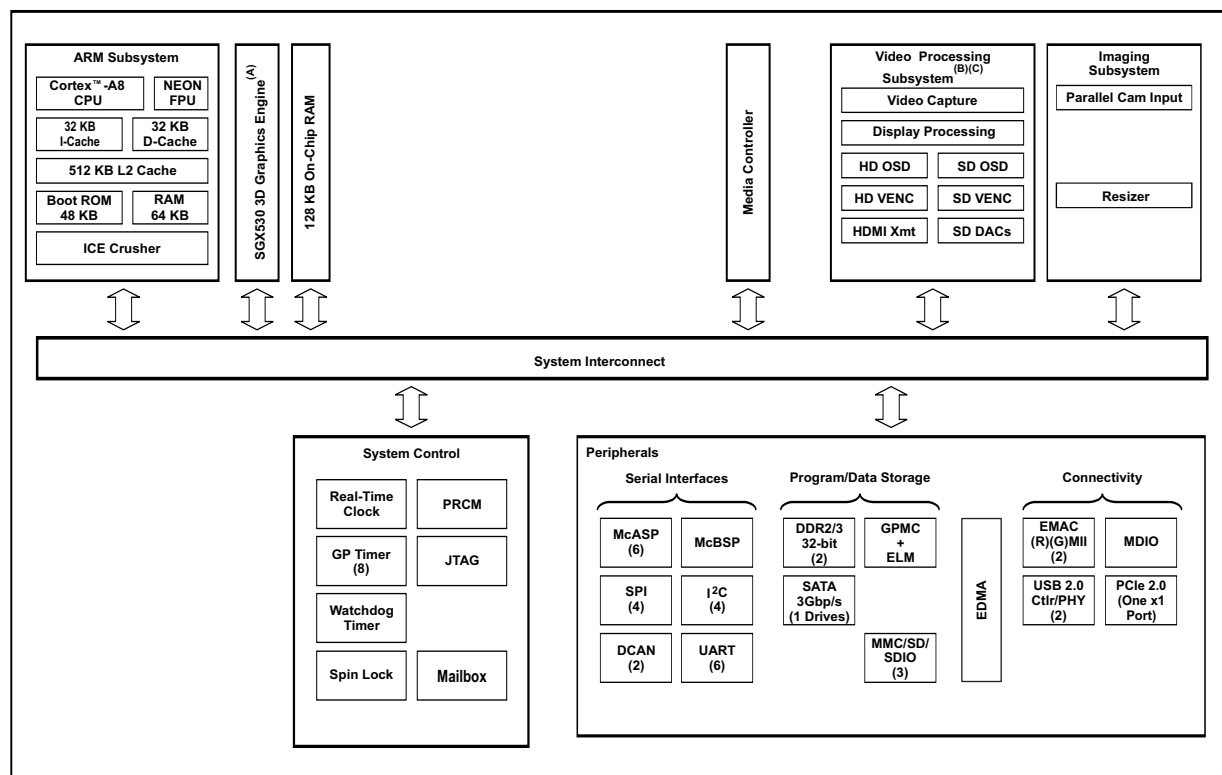
Figure 1-1. AM387x Sitara ARM Processors Functional Block Diagram
