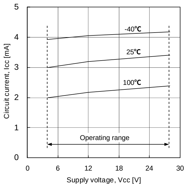
Fig.3 Circuit current
