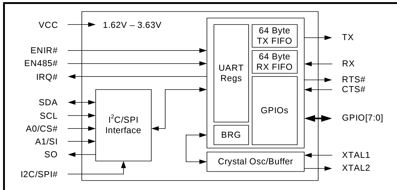
FIGURE 1. XR20M1170 BLOCK DIAGRAM
