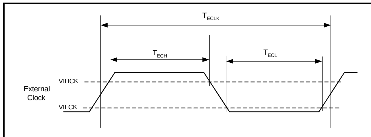
FIGURE 20. CLOCK TIMING
