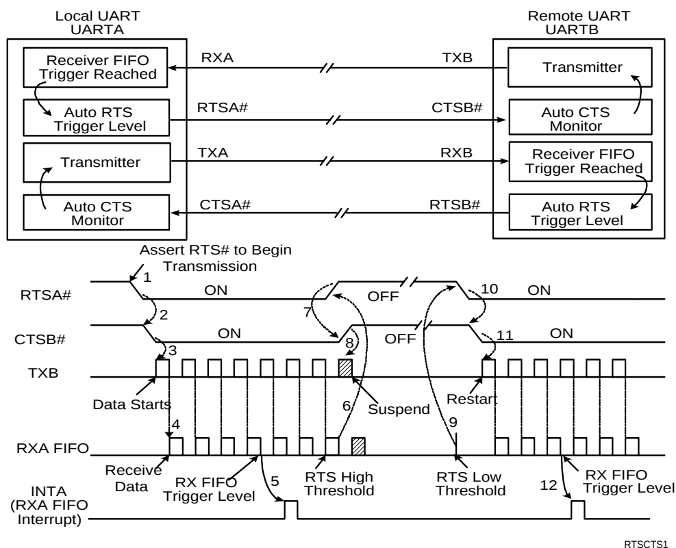
FIGURE 17. AUTO RTS AND CTS FLOW CONTROL OPERATION
