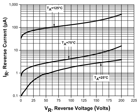
Leakage Current for CMH3-200MHV
