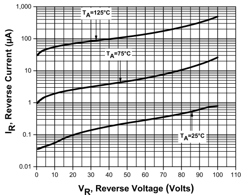
Leakage Current for CMH3-100MHV
