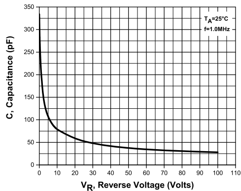
Capacitance for CMH3-100MHV
