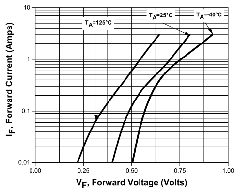
Forward Voltage for CMH3-150MHV
