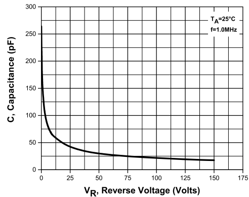
Capacitance for CMH3-150MHV
