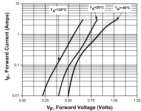
Forward Voltage for CMH3-200MHV
