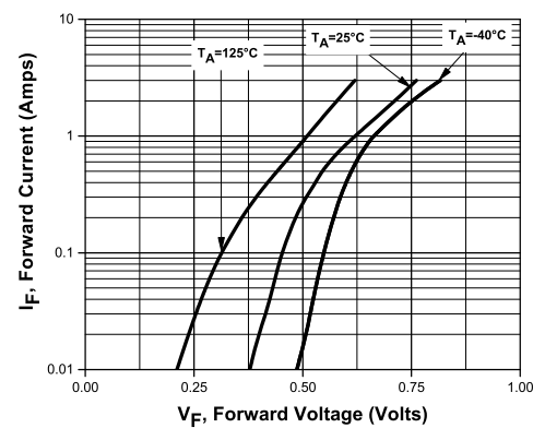
Forward Voltage for CMH3-100MHV
