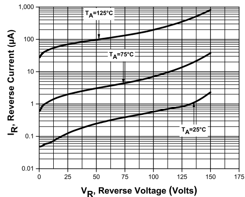
Leakage Current for CMH3-150MHV
