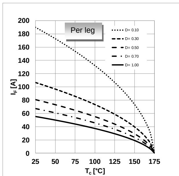
Figure 2. Diode forward current per leg as function of temperature, parameter: T_j \leq 175^\circ\text{C} , R_{th(j-c),max} , D =duty cycle, V_{th} , R_{diff} @ T_j=175^\circ\text{C}
