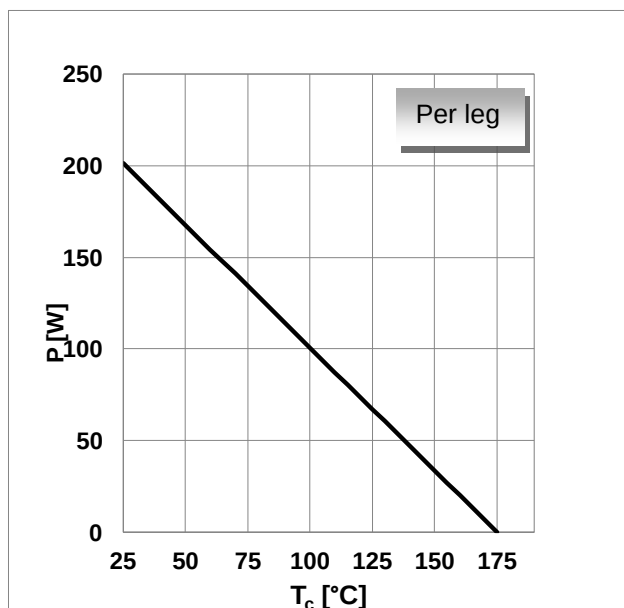
Figure 1. Power dissipation per leg as function of case temperature, P_{tot}=f(T_c) , R_{th(j-c),max}
