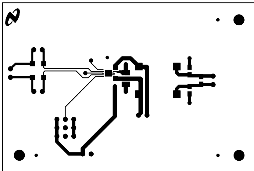
Figure 43. Bottom Layer
