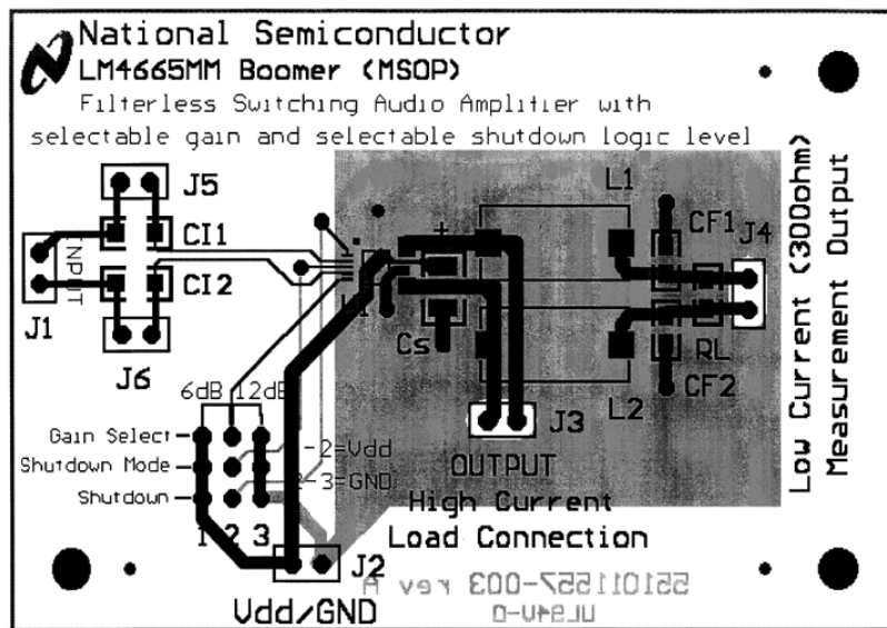
Figure 36. Composite View
