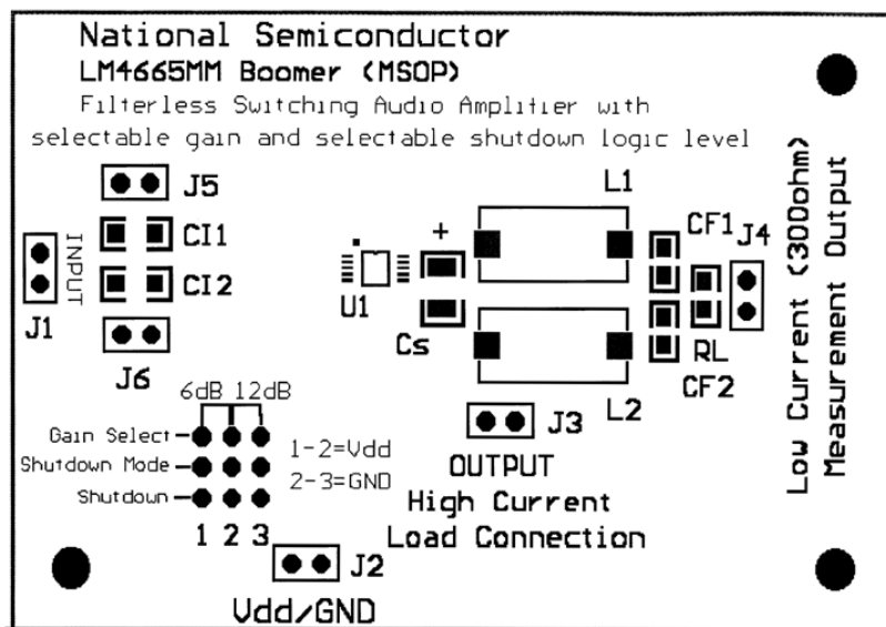
Figure 37. Silk Screen
