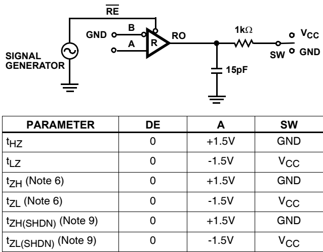
FIGURE 5A. TEST CIRCUIT
