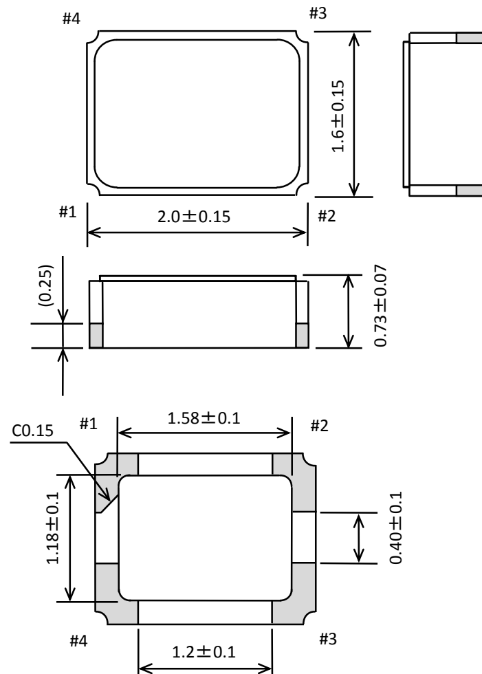
[ 7 ] Outline drawing unit:mm
