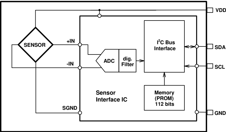
Figure 1: Block diagram of MS5805-02BA
