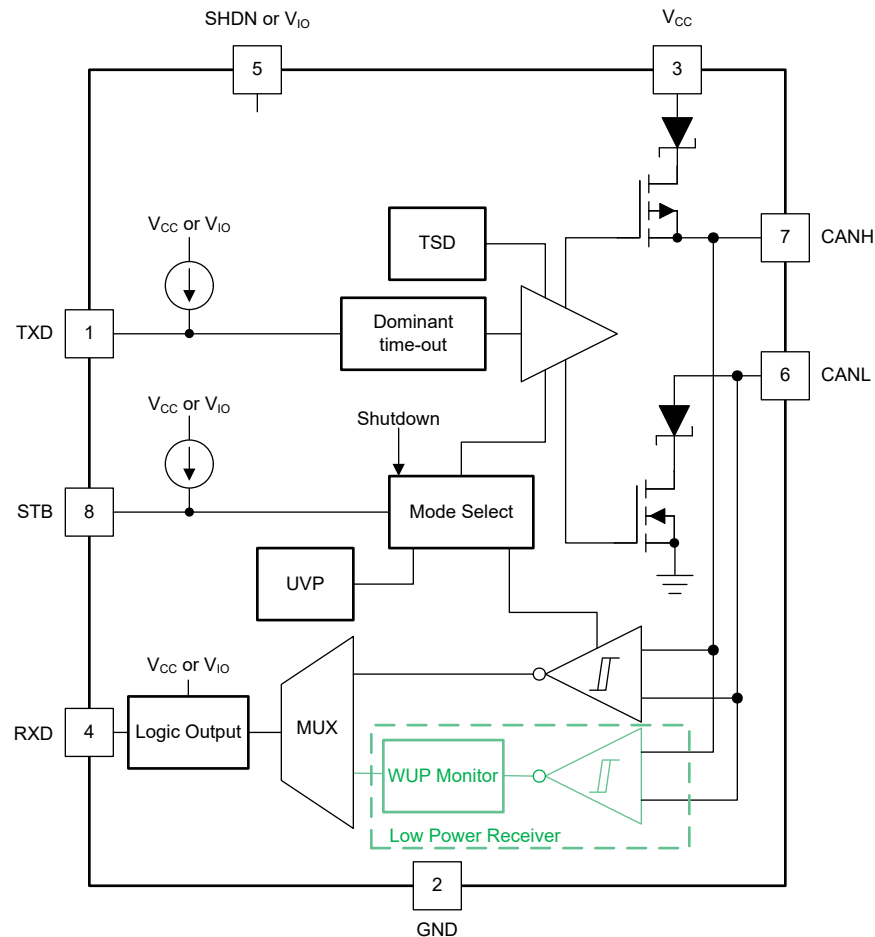
Figure 8-1. Block Diagram
