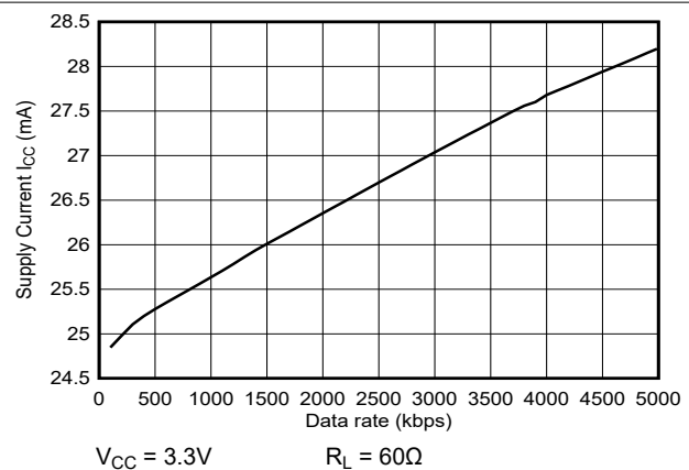
Figure 6-6. I_{CC} vs Data Rate
